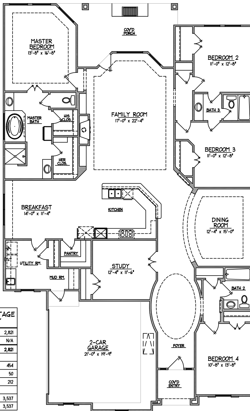
FLOOR PLAN 48'-6" x 79'-4"
