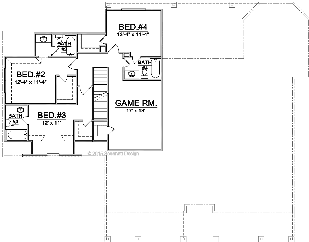
SECOND FLOOR
